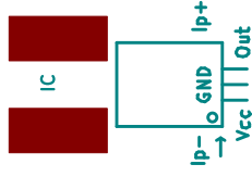
Allegro_HallSensor_Package-CB-PSS_05Jun2012
