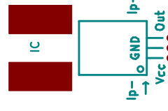
Allegro_HallSensor_Package-CB-PSF_05Jun2012
