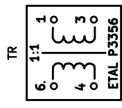
NF-Transformer_P3356_ETAL_RevA_30Aug2012
