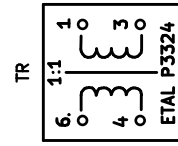
NF-Transformer_P3324_ETAL_RevA_30Aug2012
