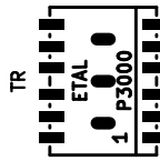
NF-Transformer_P3000_ETAL_HandSoldering_RevA_31Aug2012
