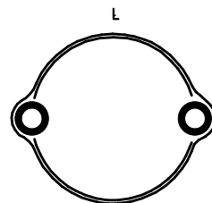
Choke_15uH/12A_DM27mm_C&D_Bobin_Type_No1410312
